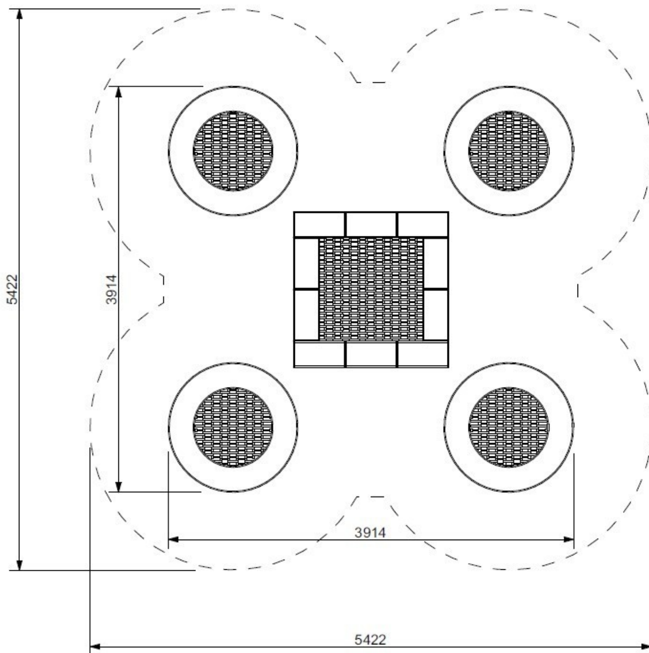
Att. 1 . Trampoline dimensions.
