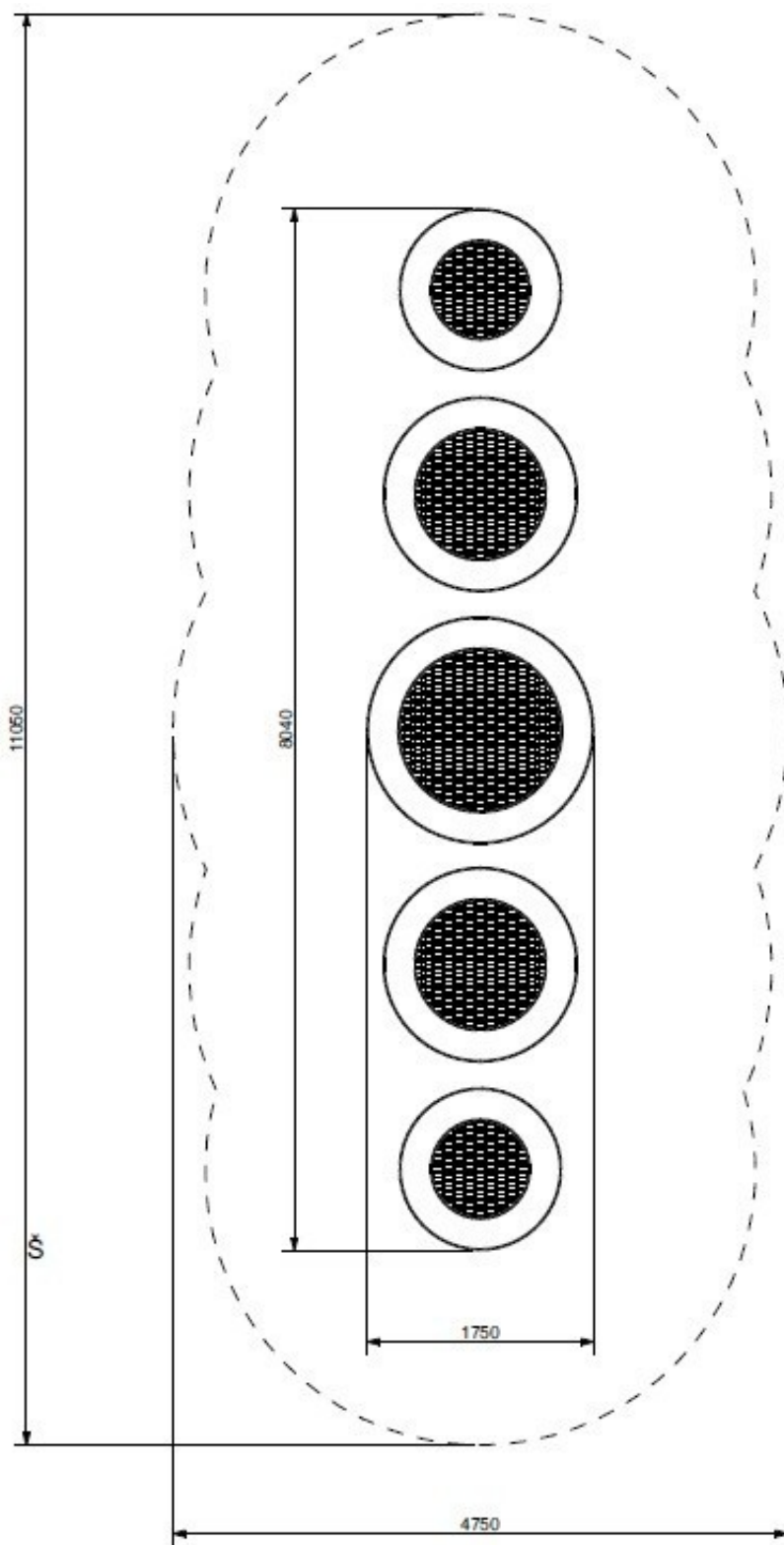
Att. 1 . Trampoline dimensions.
